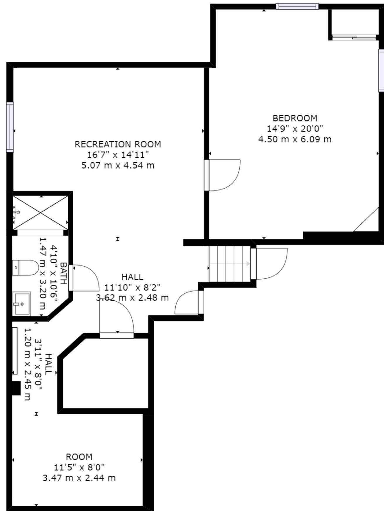
FLOOR 1
