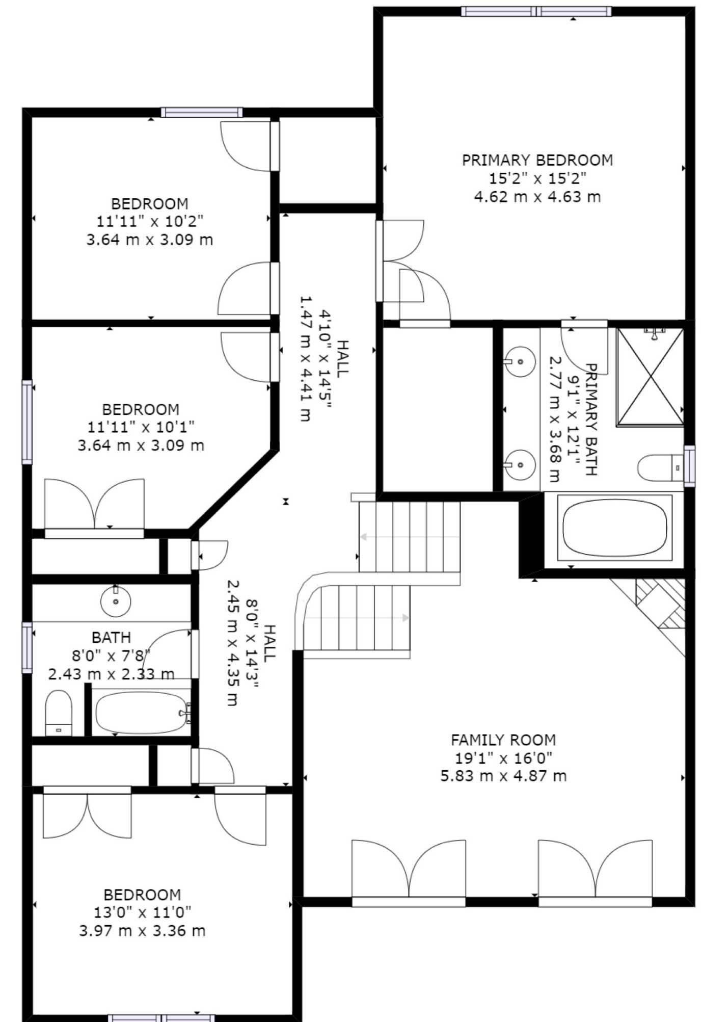
FLOOR 3
