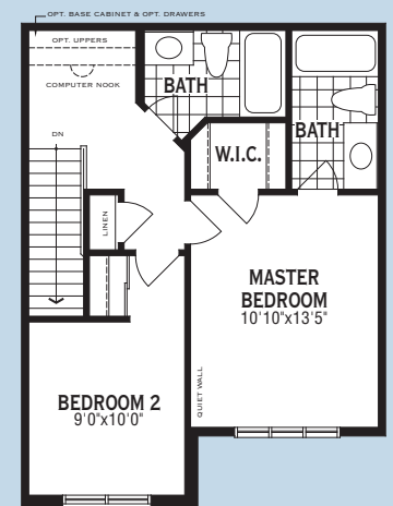
Opt. Third Floor Plan 2 Bedroom w/Master Ensuite
